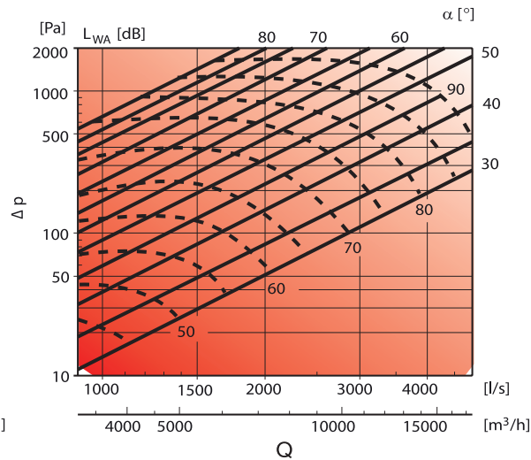
AKH Ø630
