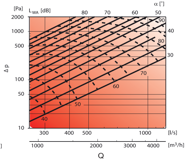
AKH Ø630
