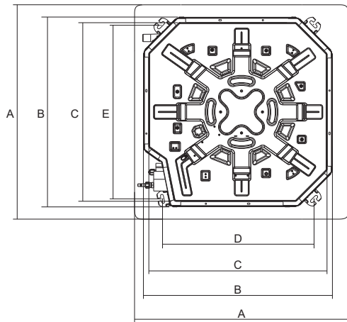
■ GMV-ND80T/C-T - GMV-ND140T/C-T
