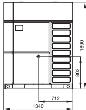
■ GMV-VQ400WM/C-X, GMV-VQ450WM/C-X
