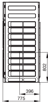
■ GMV-VQ400WM/C-X, GMV-VQ450WM/C-X
