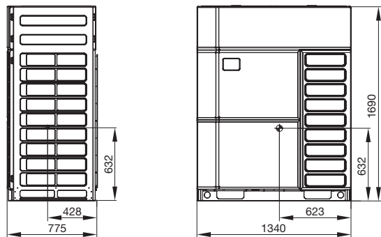
■ GMV-504WM/H-X, GMV-560WM/H-X
