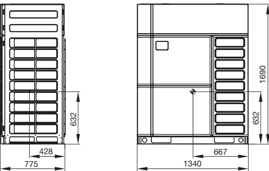
■ GMV-400WM/H-X, GMV-450WM/H-X
