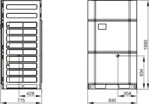
■ GMV-224WM/H-X, GMV-280WM/H-X
