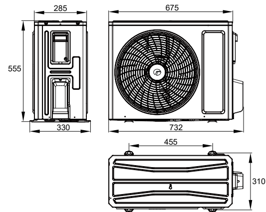
■ GWH09AVCXB-K6DNA1B/O
