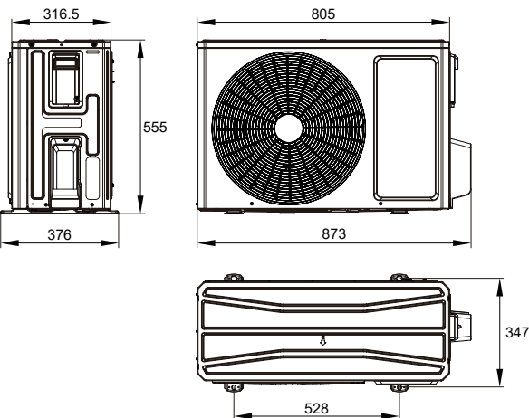
■ GWH18AVDXE-K6DNA1A/O
