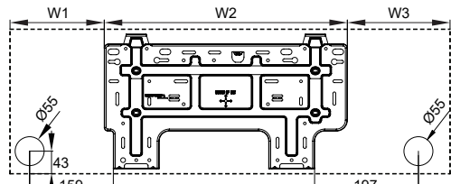
■ GWH09AVCXB-K6DNA1B - GWH12AVCXD-K6DNA1A
