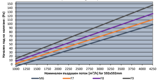
V-Compact Filter "High Temp."
