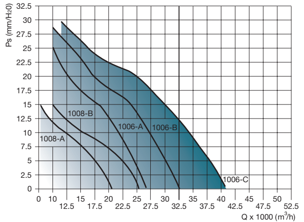
CAF / CAF ATEX 1000 - 6/8p
