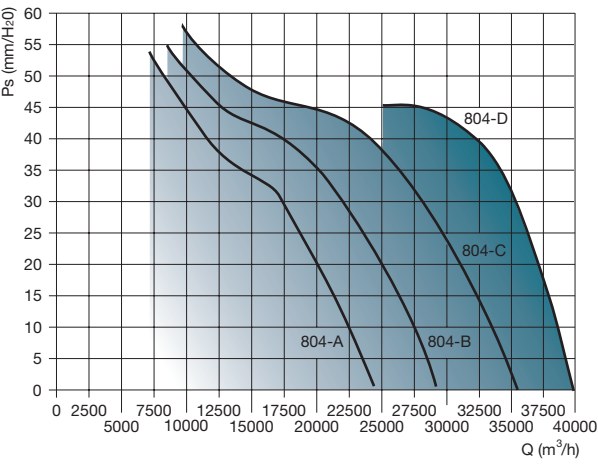
CAF / CAF ATEX 800 - 4p
