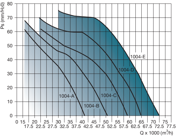
CAF / CAF ATEX 1000 - 4p
