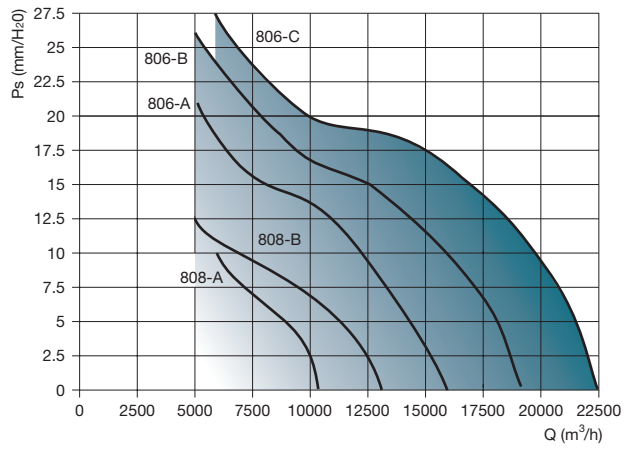
CAF / CAF ATEX 800 - 6/8p
