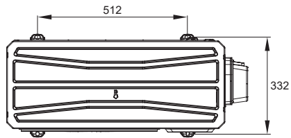
■ GWHD(18)NK6OO(LC)(LH)
