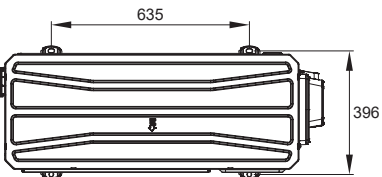
■ GWHD(36)NK6OO(LC)(LH) - GWHD(42)NK6OO(LC)(LH)
