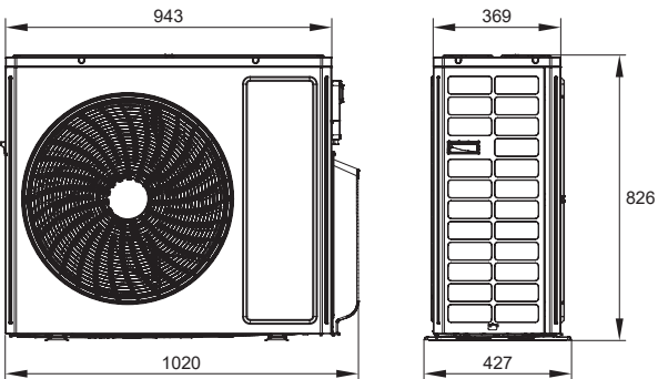
■ GWHD(18)NK6OO(LC)(LH)
