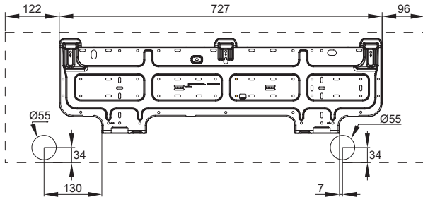
■ GWH09AECXB-K6DNA1A(I) - GWH12AECXD-K6DNA1A(I)
