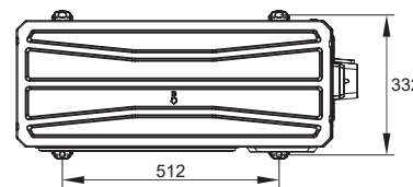
■ GWH12AECXD-K6DNA1A(O)
