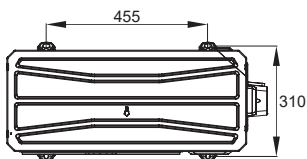
■ GWH09AECXB-K6DNA1A(O)
