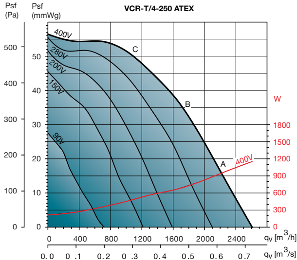
VCR-T/4-250 ATEX
