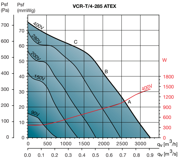
VCR-T/4-285 ATEX
