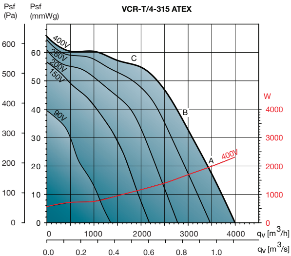
VCR-T/4-315 ATEX
