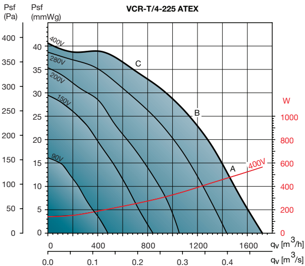
VCR-T/4-225 ATEX
