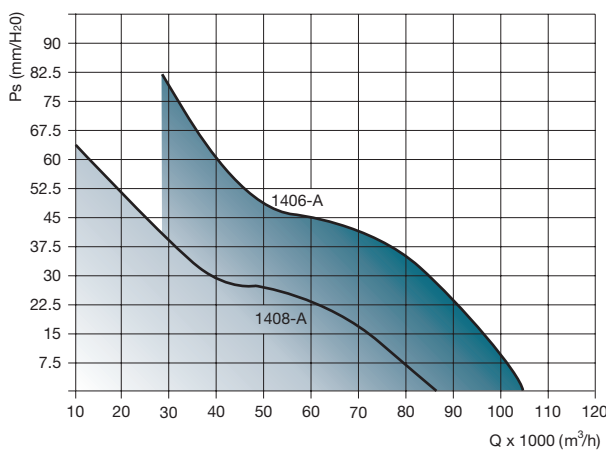
CAF / CAF ATEX 1400 - 6/8p
