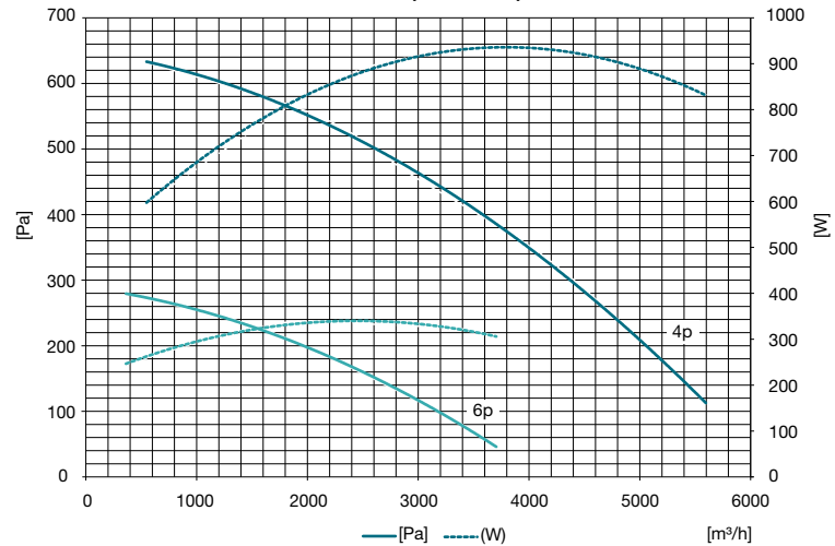
DFA 500 4p/ DFA 500 6p
