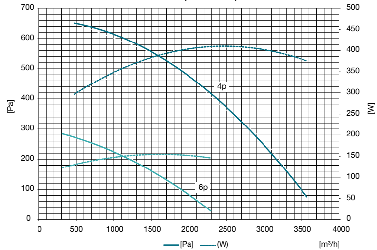
DFA 450 4p/ DFA 450 6p
