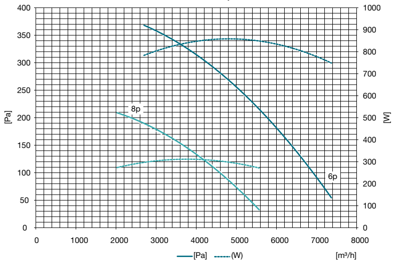
DFA 560 6/8p
