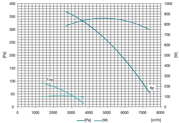
DFA 560 6/12p
