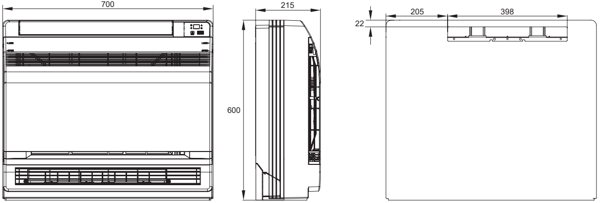
■ GEH09AAXB-K6DNA1A/I - GEH18AAXF-K6DNA1A/I
