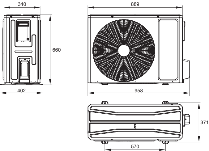
■ GEH18AAXF-K6DNA1A/O
