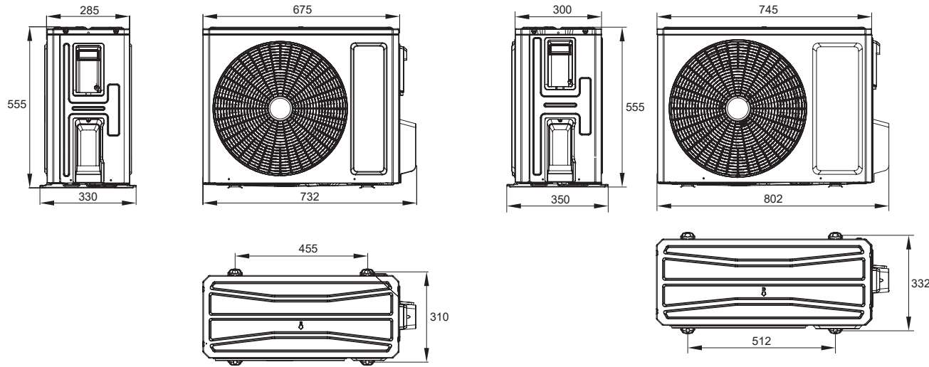
■ GEH09AAXB-K6DNA1A/O
