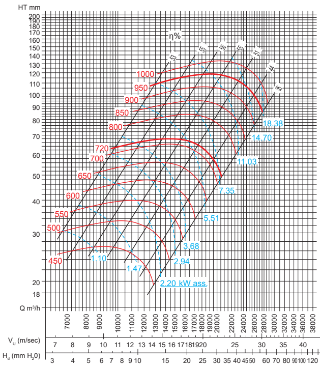
VSB 70 (50/135)
