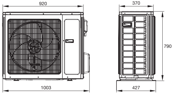
■ GWH18YE-S6DBA1A(I) - GWH24YE-S6DBA1A(I)
