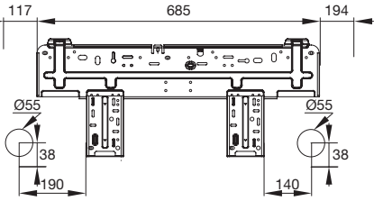
■ GWH09YD-S6DBA1A(I) - GWH12YD-S6DBA1A(I)
