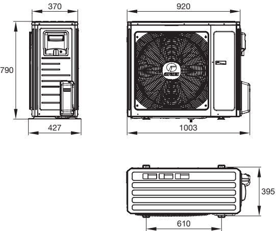
■ GWH24YE-S6DBA1A(O)
