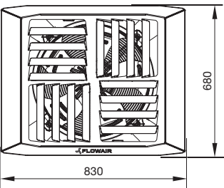
■ LEO D XL BMS | LEO DT XL | LEO D XL
