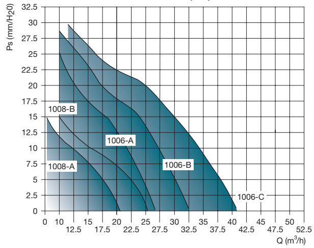
RING 1000 - 6p - 8p
