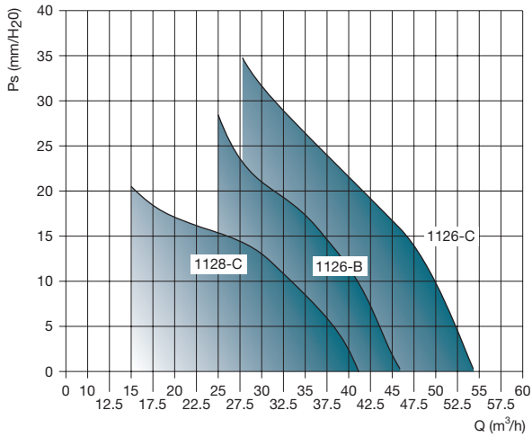
RING 1120 - 6p - 8p
