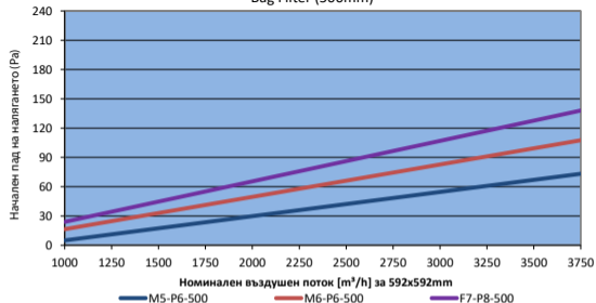
Bag Filter (500mm)
