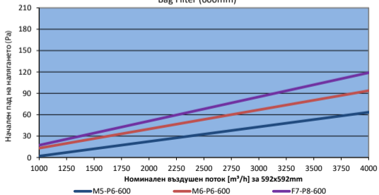
Bag Filter (600mm)
