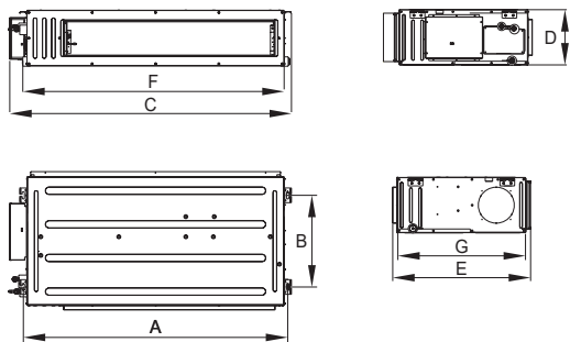
■ GMV-NDX125P/A-T, GMV-NDX140P/A-T
