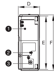
■ GUD71PH1/A-S - GUD160PHS1/A-S
