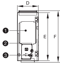
■ GUD35P1/A-S - GUD50PS1/A-S
