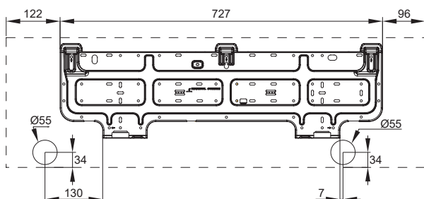
■ GWH09AECXB-K6DNA1A(I) - GWH12AECXD-K6DNA1A(I)
