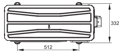
■ GWH12AECXD-K6DNA1A(O)
